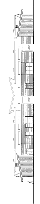
PROPOSED WEST ELEVATION - showing rear of New Extension
